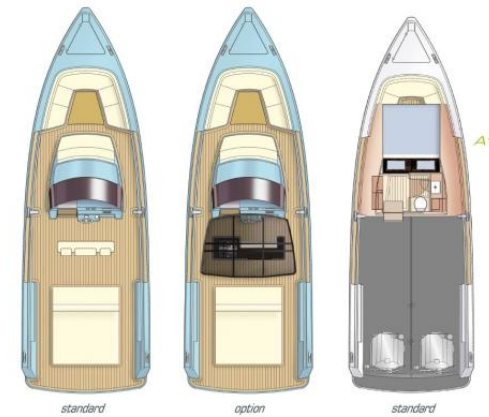
FJORD 36 open | exterior & interior layouts
