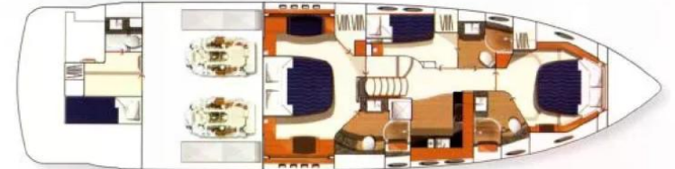
Lower accommodation layout
