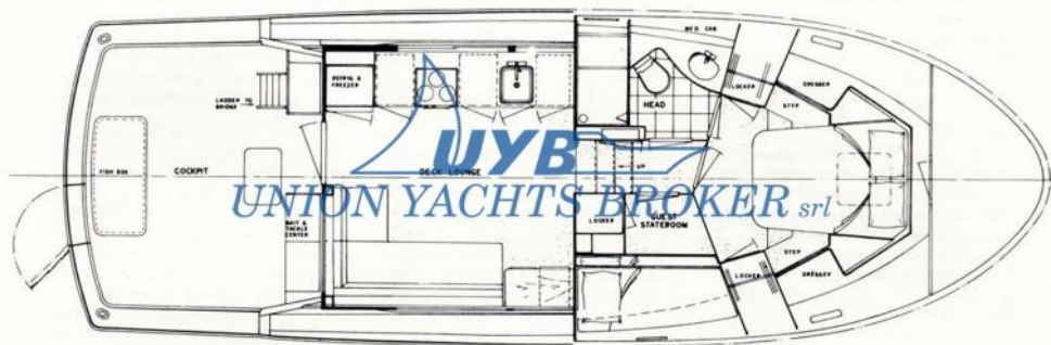
Hatteras 41 Convertible
