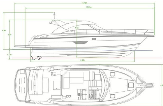
R4400SY Principal Dimensions ISO 8666:2002
