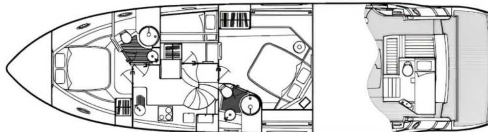
Lower deck
